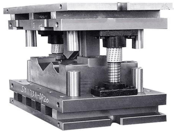
Sheet Metal Stamping Tool
